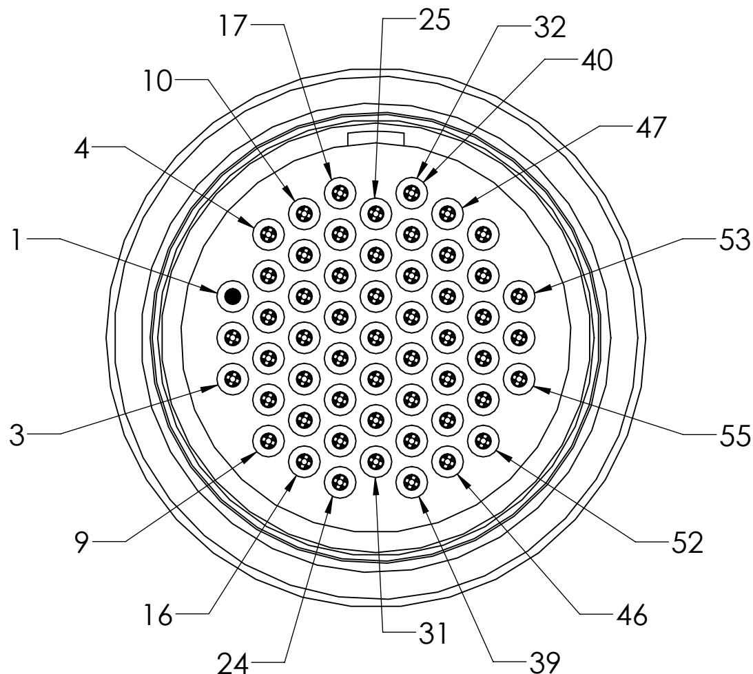
INSULATION COLOR POSITIONS VIEW A-A (MATING FACE) SCALE 5:1
